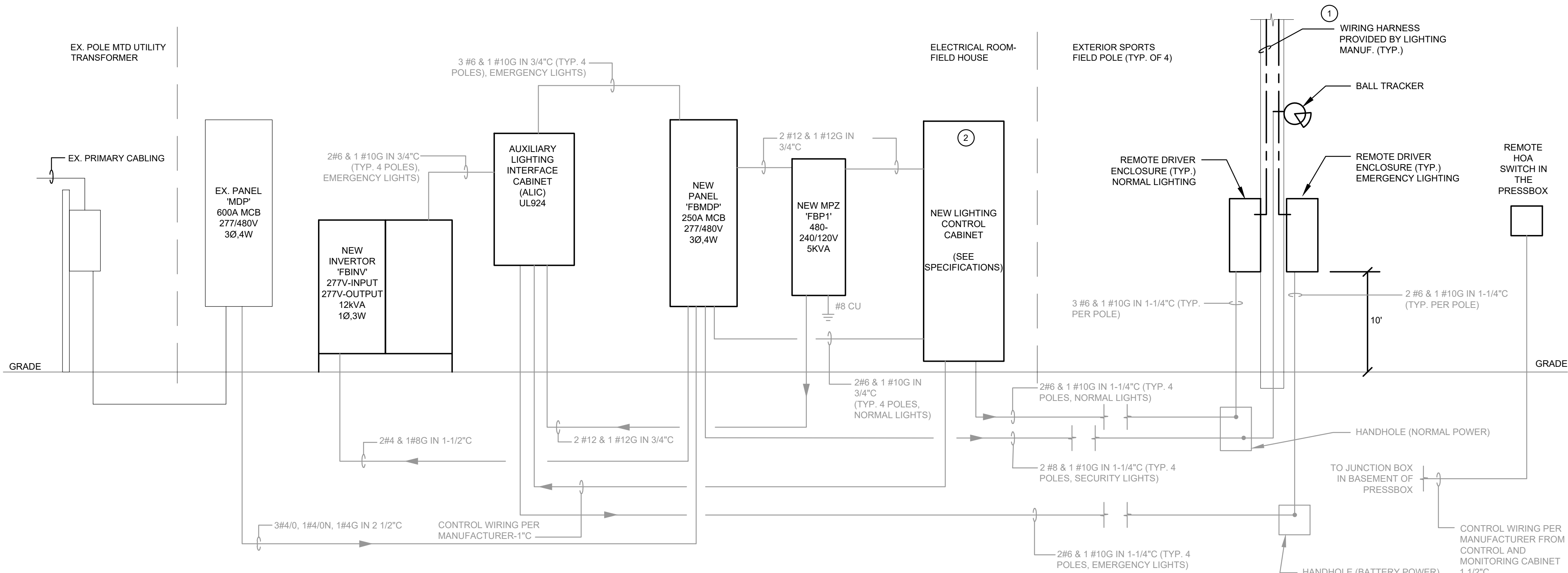
1 CARY HIGH SCHOOL FOOTBALL STADIUM LIGHTING - RISER DIAGRAM SCALE: NTS
